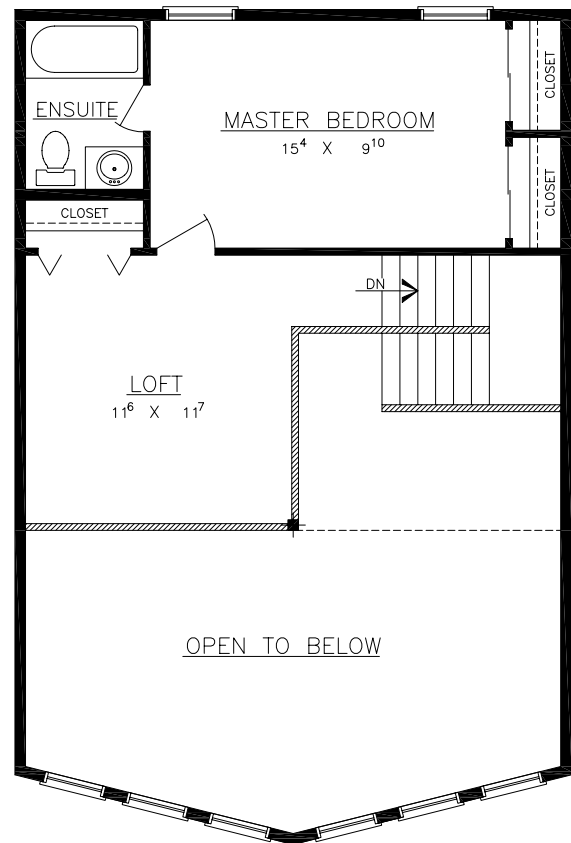
SECOND FLOOR AREA = 409 S.F.
