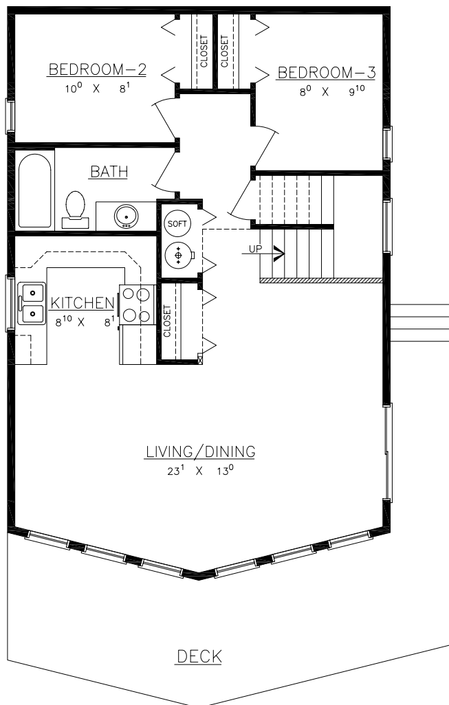
MAIN FLOOR AREA = 828 S.F.
